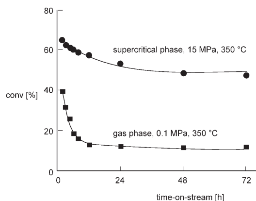
Figure 2. The catalyst lifetime: Influence of time-on-stream on the catalytic activity as a function of conversion of ortho -methylation of phenol under supercritical and gas phase conditions for several days.
