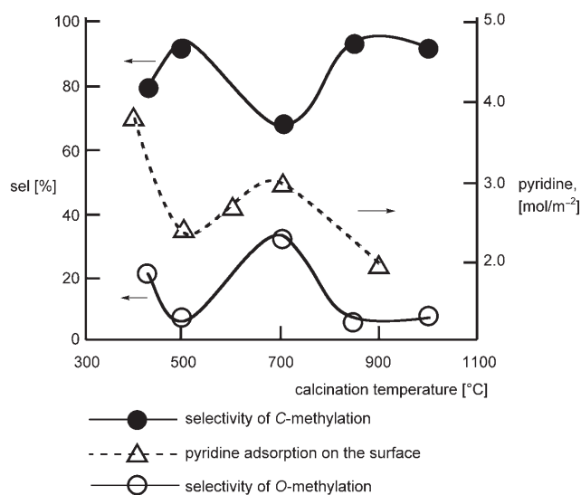
Figure 1. Calcination temperature effect on chemoselectivity over ZrO 2 catalysts.
